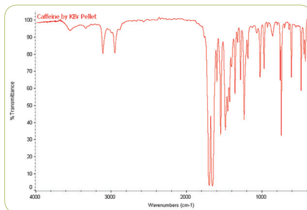
FTIR spectrum of caffeine in KBr pellet made using the PIKE CrushIR Hydraulic Press and Evacuable Pellet Press.
